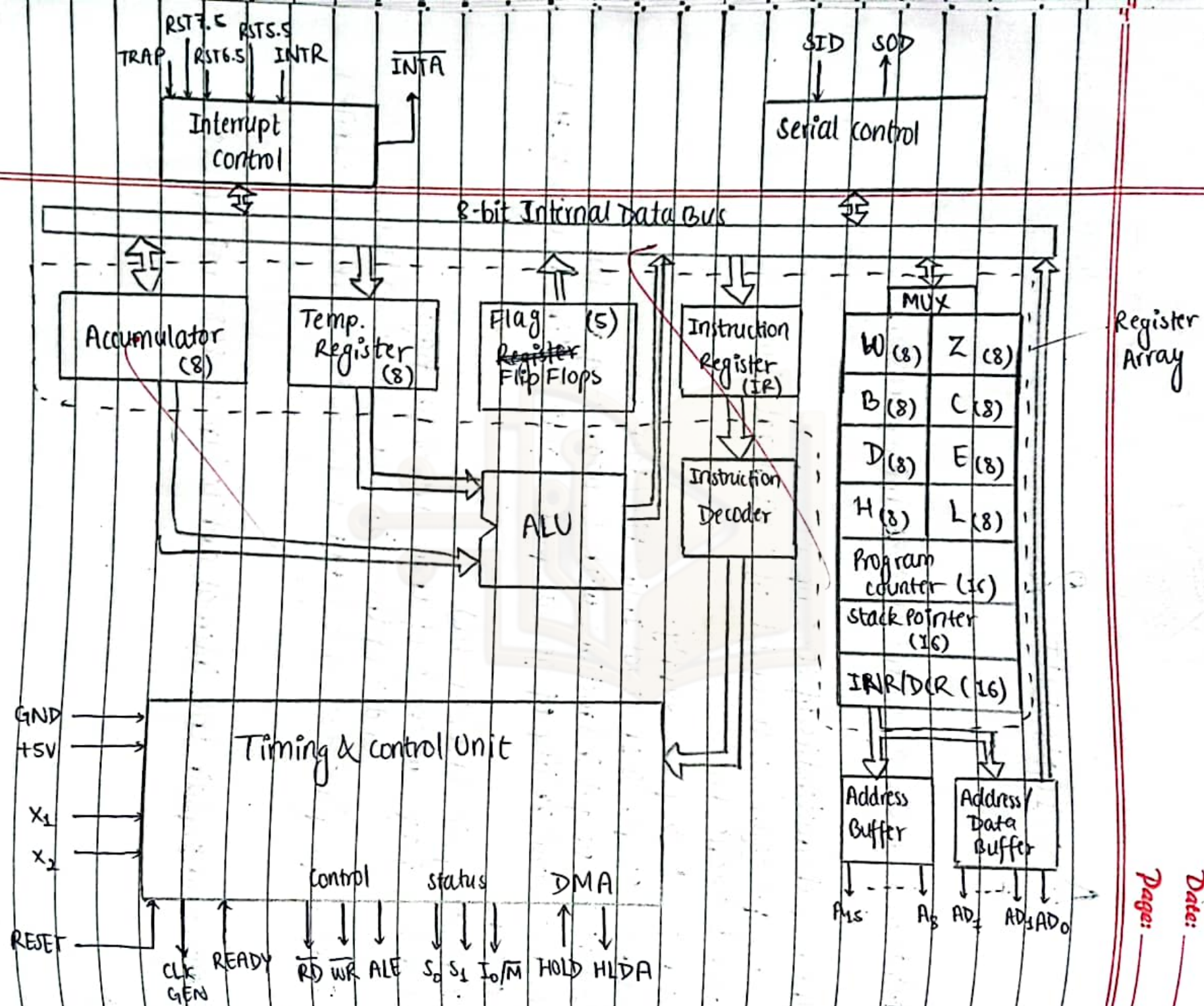
Fig. Internal Architecture of 8085 \mu P.
